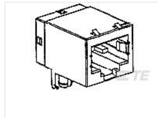
TE 产品编号5558342-1 MJ,8POS,R/A,CAT5,SHLD,PC GND INS
