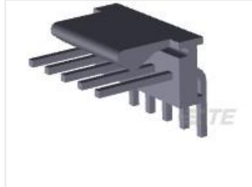
TE 产品编号640457-5 05P MTA100 HDR ASSY SQ R/A F/L
