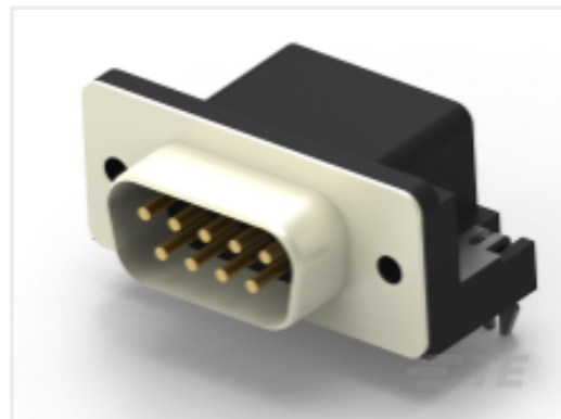
TE 产品编号2301843-1 AMPL PLUG HD20, R/A, 9P, B/L,4-40 INS
