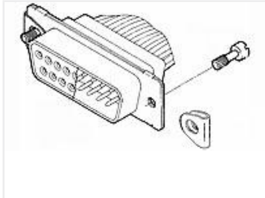
TE 产品编号211883-5 SCREW RETAINER KIT,AMPLITE
