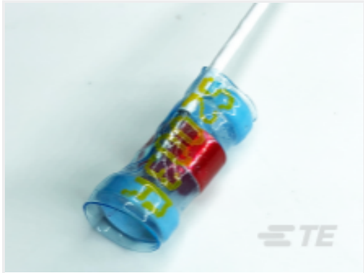
TE 产品编号CP1854-000 S200-1-W2-22-9-TC
