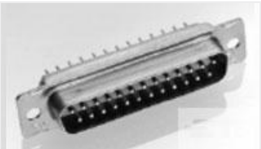
TE 产品编号1757823-9 AMPLIMITE,ASY,PLUG,STD,90,ZN,3,CT
