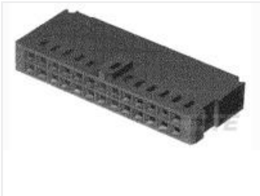
TE 产品编号102387-5 24 MODIV HSG COMP DR .100 POL
