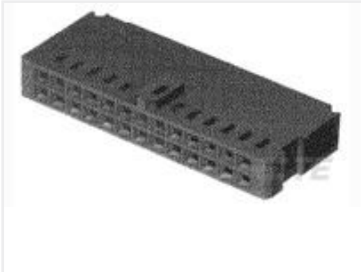
TE 产品编号102387-1 10 MODIV HSG COMP DR .100 POL
