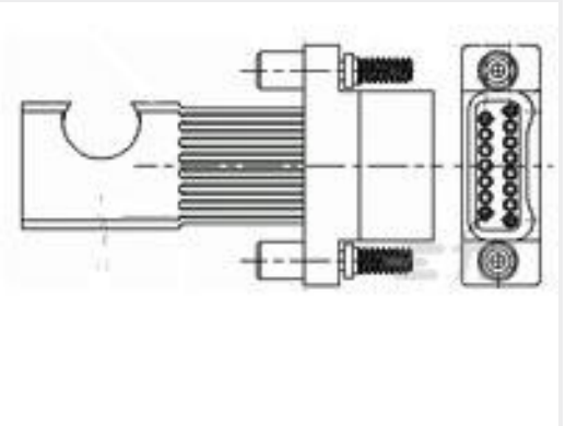
TE 产品编号1-1589478-0 STM051B5 = SMT CONN
