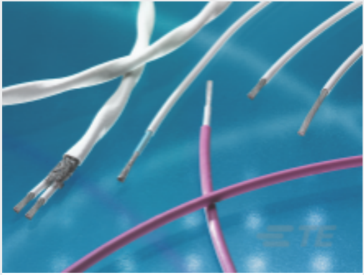
TE 产品编号CAT-55M-TC-TP Twisted Pair Cable: Tin Coated Copper Cable, 450V Dual Wall
