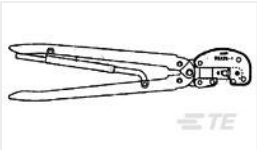
TE 产品编号59287-2 HHHT PIDG PG 12-10 ASSY
