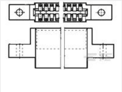
TE 产品编号2-583861-1 TW-LEAF CRP HSG. 50 POS.
