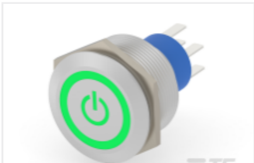
TE 产品编号2-2317658-9 AV25 DPL 3A MOVING RING POWER GREEN 24V
