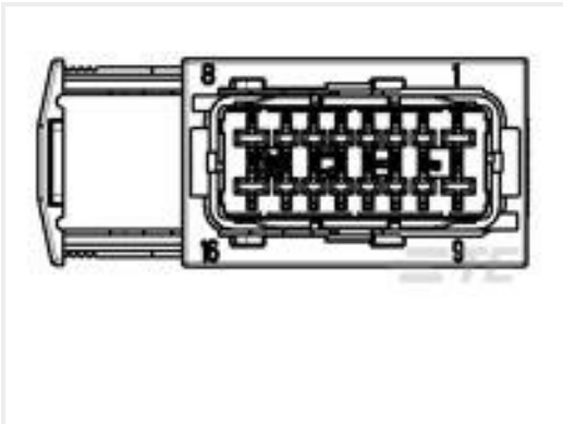
TE 产品编号185760-2 16W HYBRID RCPT HSG GREEN
