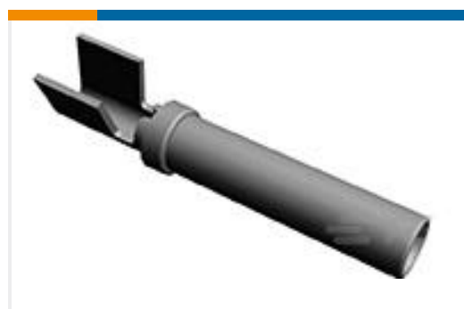
TE 产品编号776491-2 SOC, SF, SIZE 16, 14-18 AWG, NO INS, NI/SN
