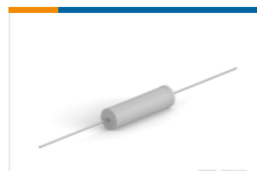
TE 产品编号2-2176414-2 7W STD M/OX 5% 150R
