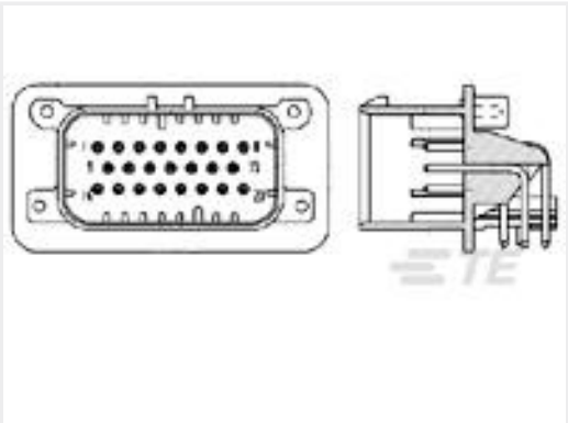
TE 产品编号1-776267-1 14POS,PIN DIA 1.3,HDR ASSY,90DEG, COD 1
