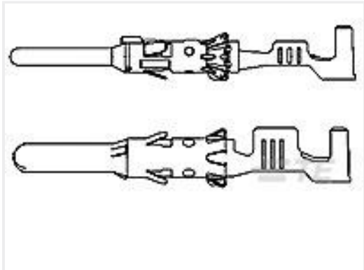
TE 产品编号1703014-1 DIA 1.5MM CONTACT PIN,ASSY
