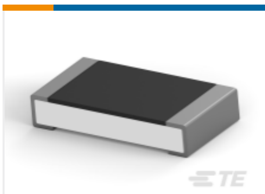
TE 产品编号6-2176388-8 RQ 1206 49R9 0.1% 10PPM 5K RL
