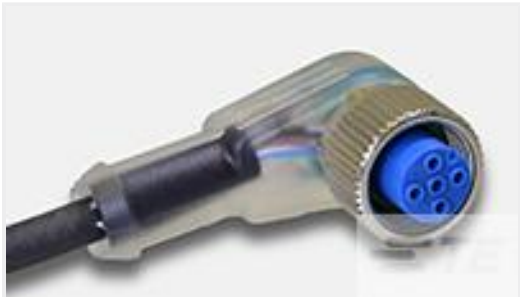
TE 产品编号 2273224-1 M12 x 1.0 angled plug 5pos shld A
