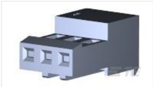
TE 产品编号3-640443-3 03P MTA100 CONN ASSY GRN
