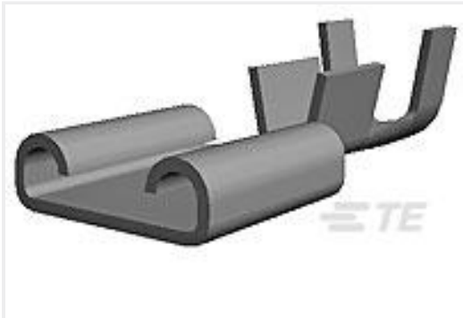
TE 产品编号5-160506-2 250 FASTON REC 20-16 AWG TPBR
