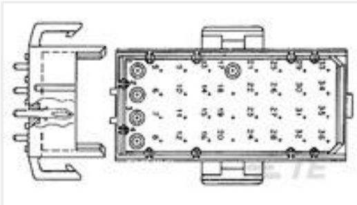
TE 产品编号640505-1 24P MR HDR ASSY V0
