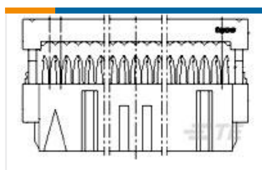
TE 产品编号2-215915-6 AMP-LATCH 15.2 HIGH TAPE
