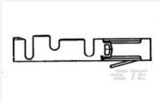
TE 产品编号281556-2 20AWG MOD 2 CRIMP TIN PLATE
