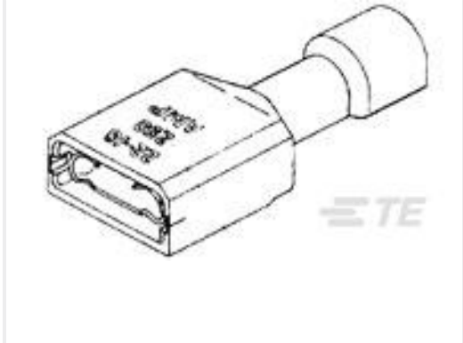
TE 产品编号2-520083-2 ULTRA-FAST .110/.125 ASY REC 22-18 TPBR
