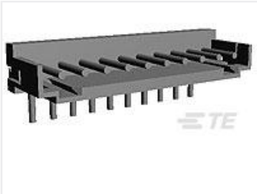
TE 产品编号292253-5 CT CONN MT HDR ASSY H 5P NAT
