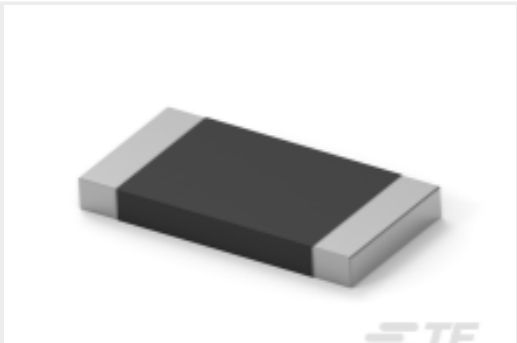
TE 产品编号4-2176422-1 TLRP 2512 3.0W R091 1% 25PPM 4K RL
