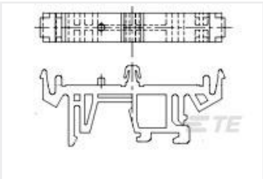
TE 产品编号6-1437661-4 TKAD=TRK ADPT. 640054900
