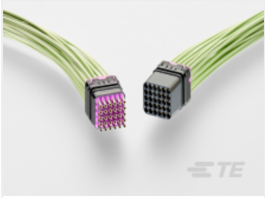
TE 产品编号ZPF00000000203398 DMC-MR 30-23 PC
