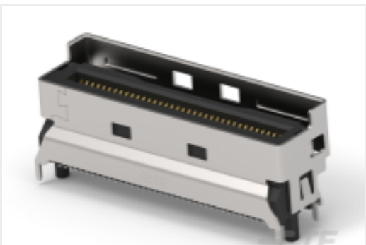
TE 产品编号2379397-6 MCIO INTERGRATED CONN, V/T,8X, SMT TYPE
