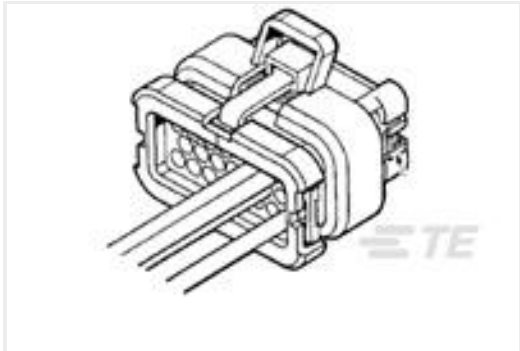
TE 产品编号770680-2 23POS,AMPSEAL,SOC HSG ASSY,SLD, COD 2
