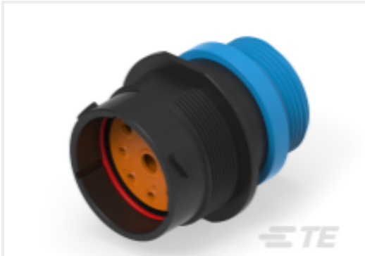
TE 产品编号HDP24-24-9PE-L015 REC, 9P, BLK, E, THD, 4/8/12, P
