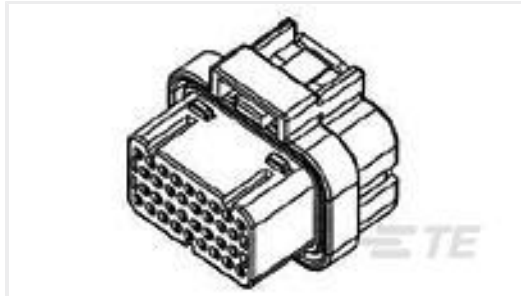
TE 产品编号1473416-2 SUPER SEAL 26POS PLUG ASSY
