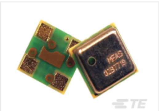
TE 产品编号MS563702BA03-50 2 BAR INDUSTRIAL ALTIMETER SENSOR
