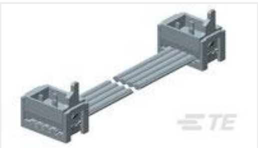
TE 产品编号2205062-2 CA MICRO-MATCH MOW-MOW 8POS
