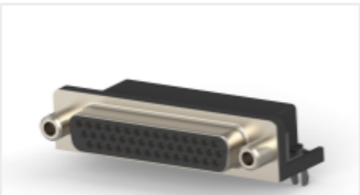
TE 产品编号2311770-1 AMPL REC, HD22, R/A, 44P, THREADED
