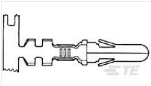
TE 产品编号350201-1 .140 DIA PIN 14-10 PTPBR
