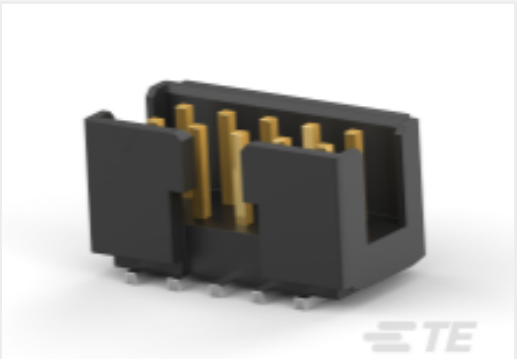
TE 产品编号1-2373376-0 10P,2MM,SHRD HDR,DRVVT,SMD,0.1 AU,TB
