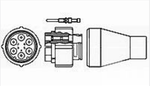
TE 产品编号863022-1 PLUG ASS'Y, 4 PIN
