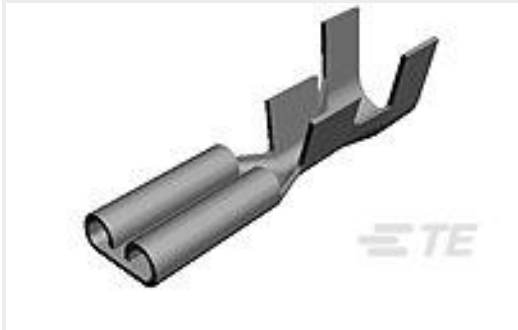
TE 产品编号42470-1 110 FASTON REC 22-18 AWG TPBR
