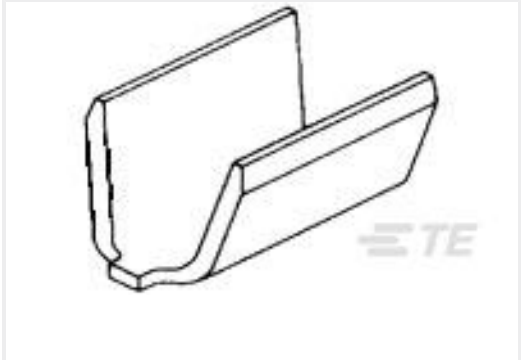
TE 产品编号42329-1 SPLICE 1200-2600 .012 NPST
