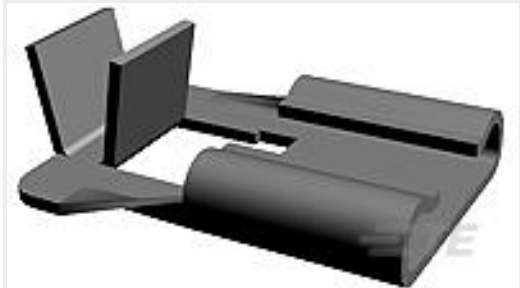
TE 产品编号63096-1 250 FASTON FLAG REC 18-14 AWG BR
