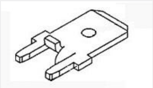
TE 产品编号1217136-1 250 FASTON,PCB TAB,TNBR
