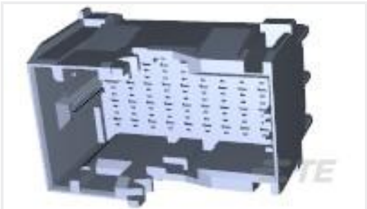
TE 产品编号1-1718492-4 1.5MM TAB HSG 36 POS ASSY
