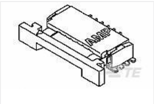
TE 产品编号2-84952-1 1MM FPC HORZ.BTTM CONT.ASS.21P
