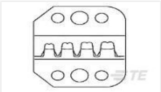
TE 产品编号91337-2 SIZE 16 PRO-CRIMPER DIE
