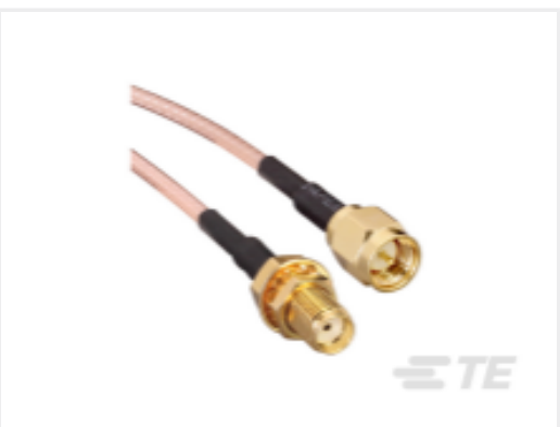
TE 产品编号CSE-SGAM-610-SGFB SMA to SMA 610mm RG316
