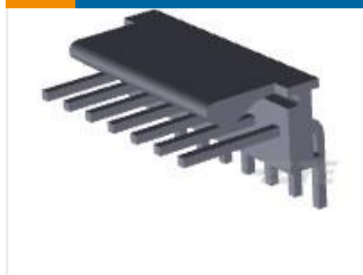
TE 产品编号640457-7 07P MTA100 HDR ASSY SQ R/A F/L
