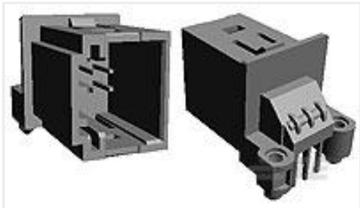
TE 产品编号953440-1 6pos MQS .63 header 90deg
