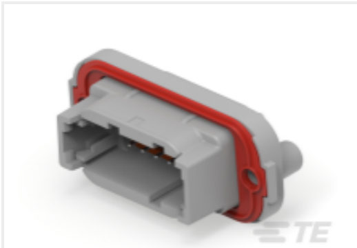
TE 产品编号DTM13-12PA HDR, 12P, GRY, RA, SN/NI/CU, A
