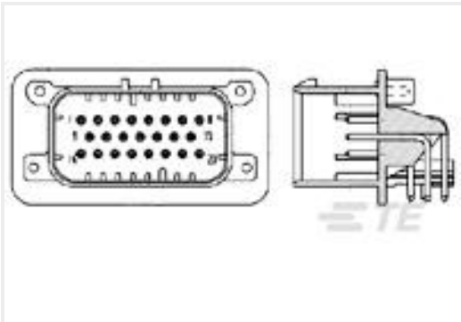
TE 产品编号776087-2 23POS,PIN DIA 1.3,HDR ASSY,90DEG, COD 2
