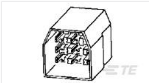
TE 产品编号151326-1 FF 250 TAB HSG 11P NYLON NAT
