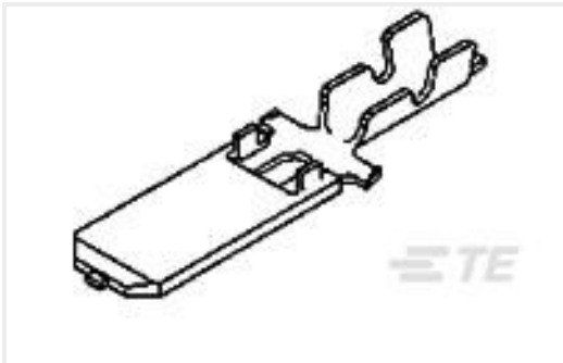
TE 产品编号170349-2 FF 250 TAB 22-20AWG TPBR WITHOUT LATCH
