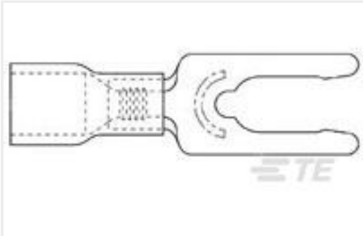
TE 产品编号52772-1 TERMINAL,BUDG SPR SPD 12-10
