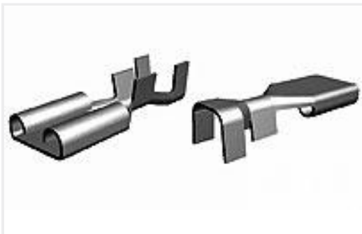
TE 产品编号63820-1 312 FASTON REC 14-10 AWG SPBR
